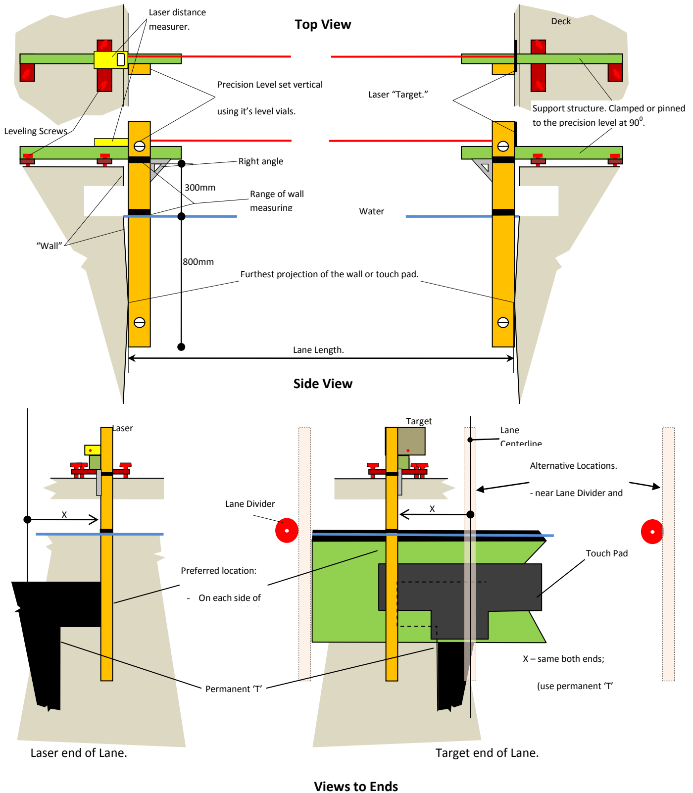
Figure 1 Using "Hand Held" Laser Measuring Equipment
